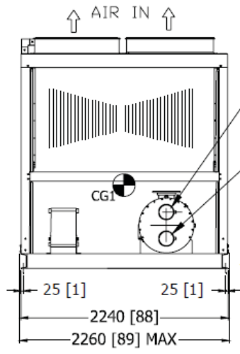
LEFT VIEW
