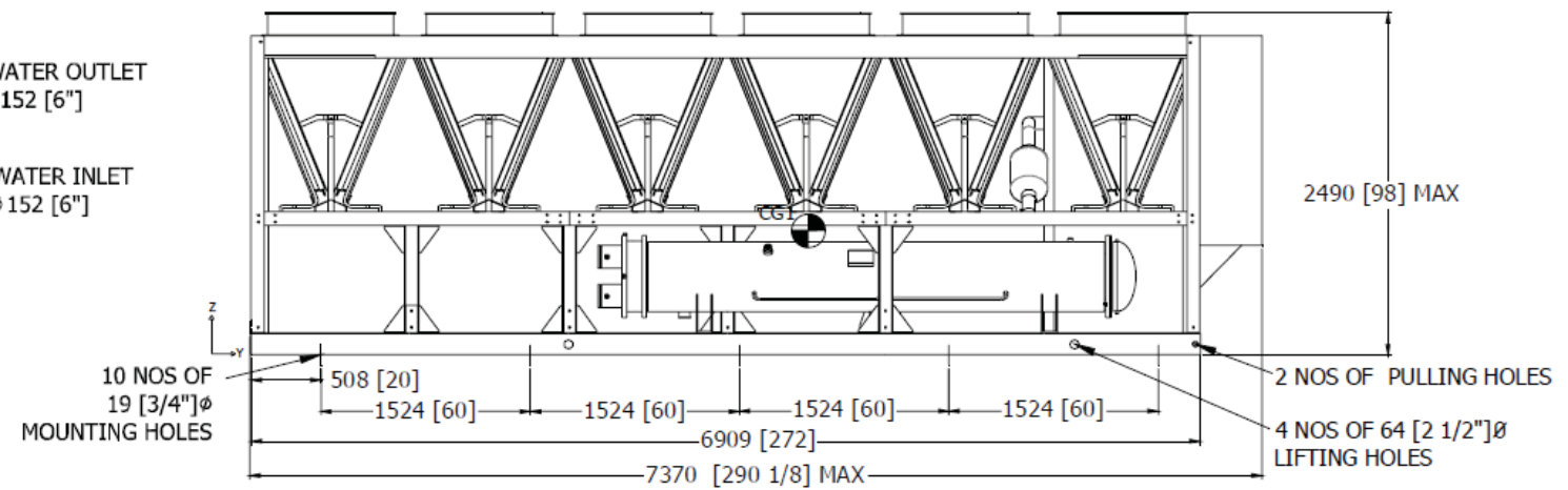
FRONT VIEW
